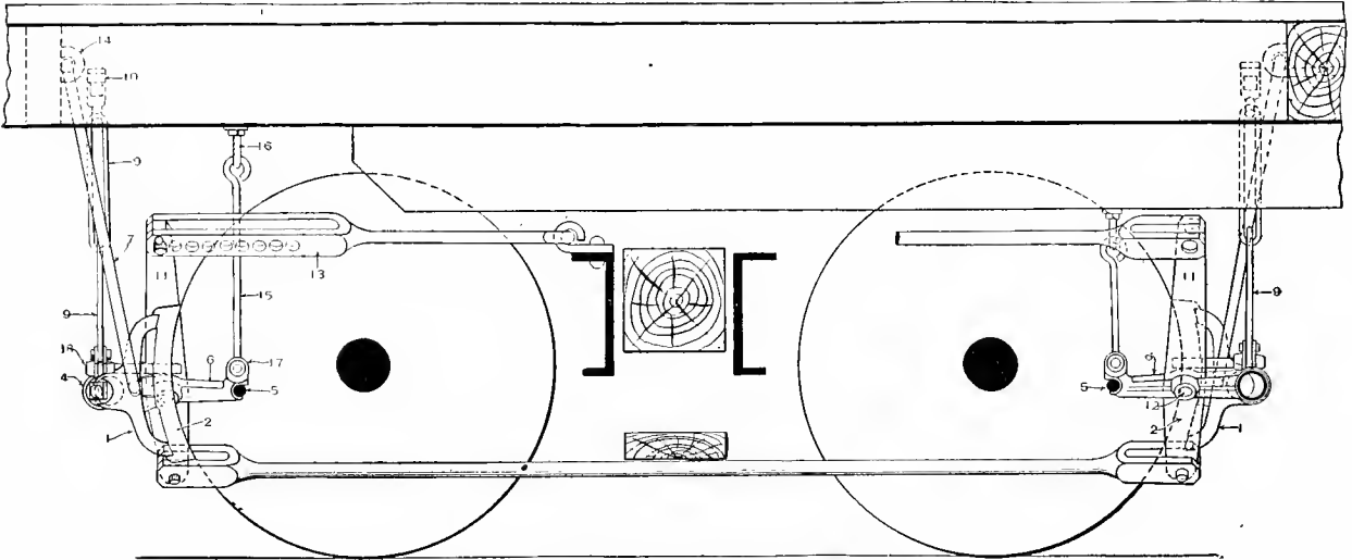
Fig. 1528. Sectional Side Elevation.
